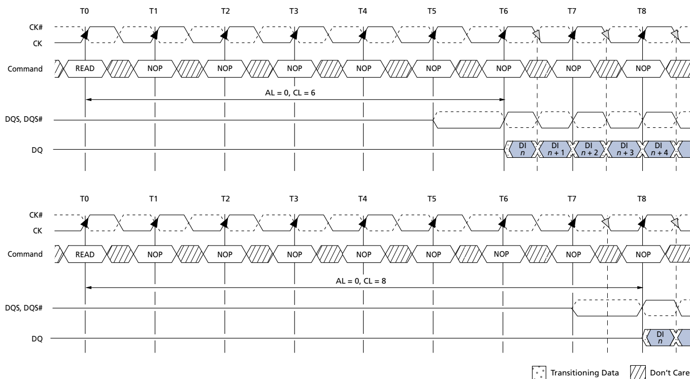
Figure 53: READ Latency
