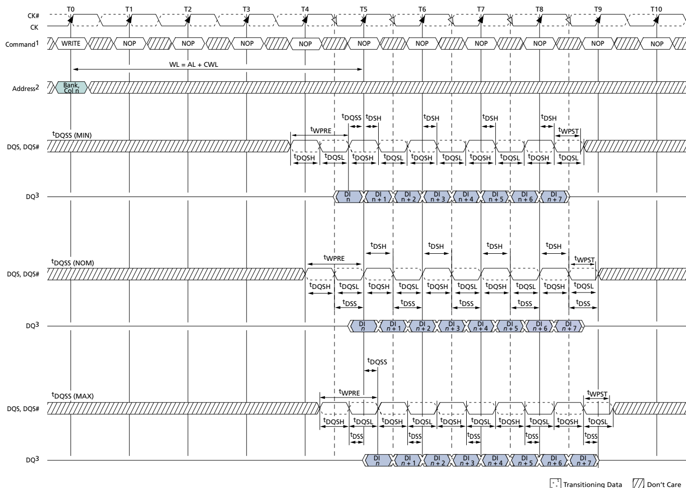
Figure 84: WRITE Burst
