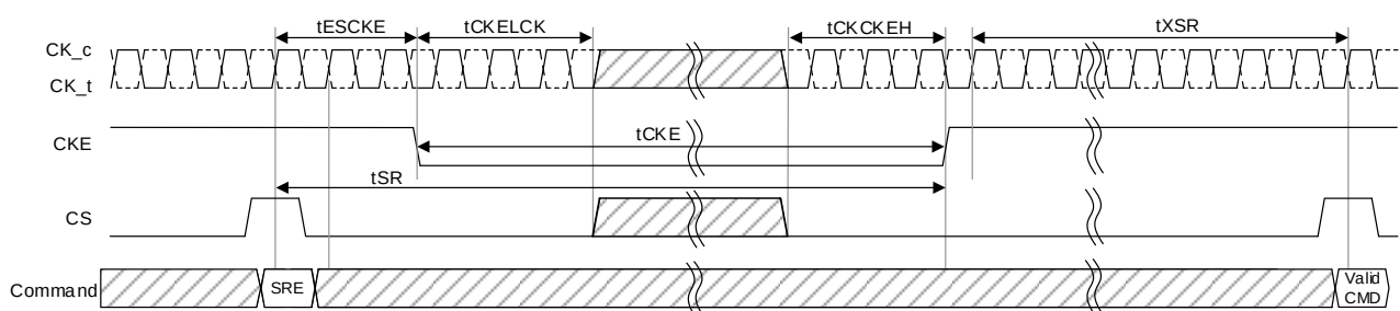
Figure 5.12. Self refresh entry and exit timing diagram
