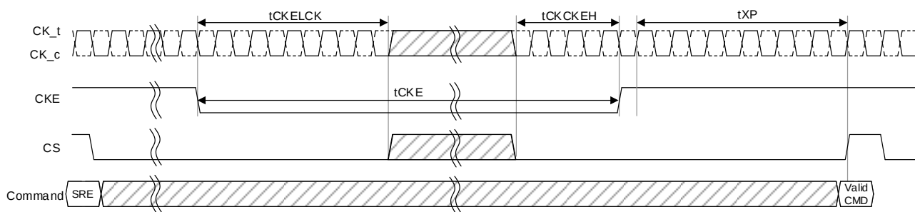
Figure 5.11. Power down entry and exit timing diagram
