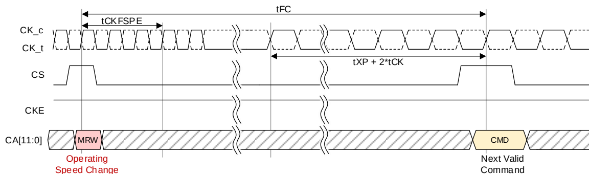
Figure 5.14. Input Clock Frequency Change Timing Diagram
