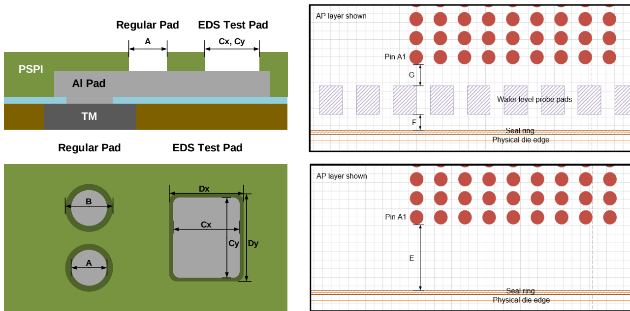
Figure 2.6. Pad Rules
