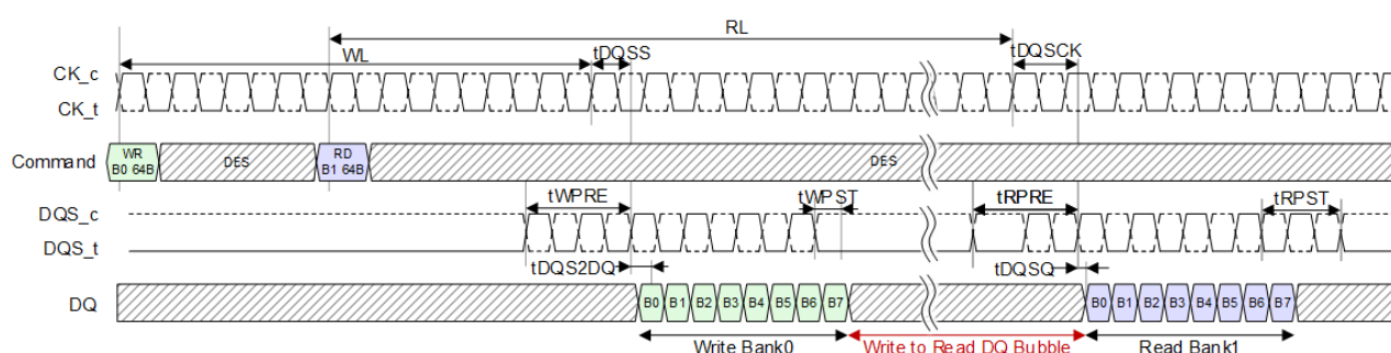
Figure 15. 64B Write followed by a 64B Read to different banks in same slice
