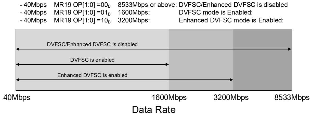
Figure 256 — The Frequency Range Supported by DVFSC and Enhanced DVFSC Mode
