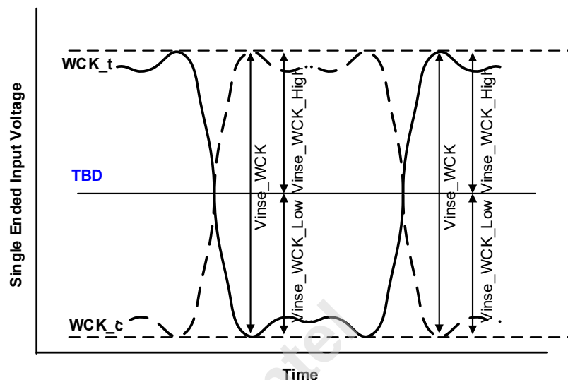
Figure 303 — WCK Single-ended Input Voltage
