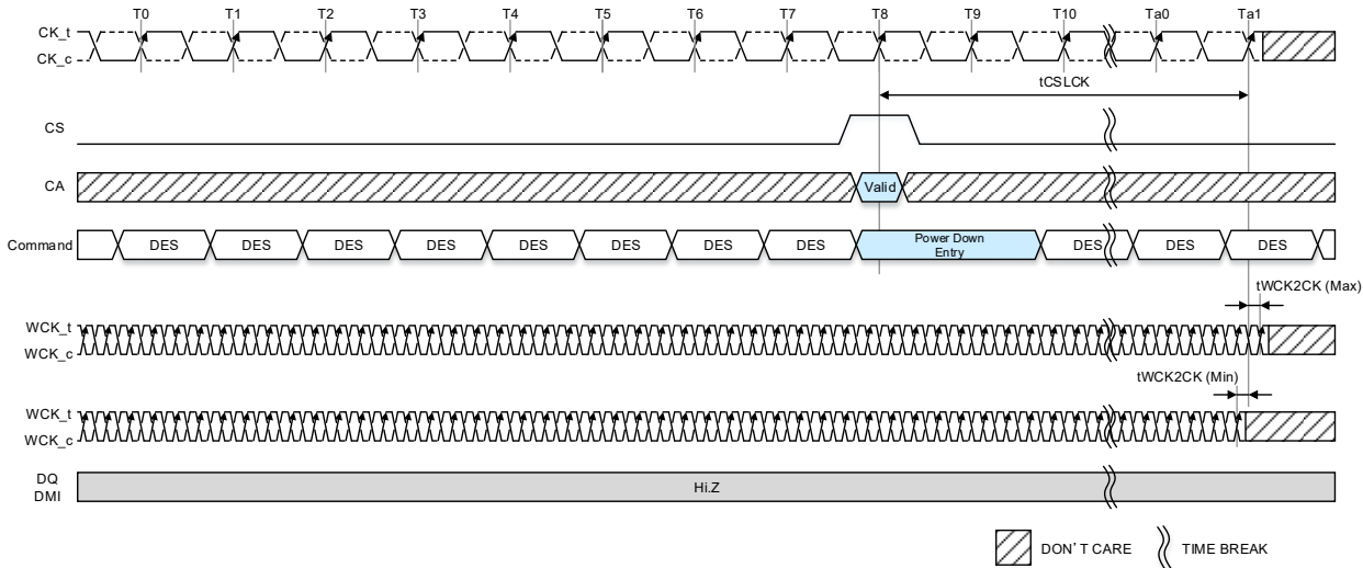
Figure 186 — Power Down Entry to CK and WCK Stop Timing
