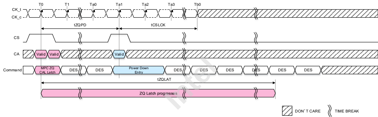
Figure 171 — Multi Purpose Command for ZQ Latch Command to Power-Down Entry
