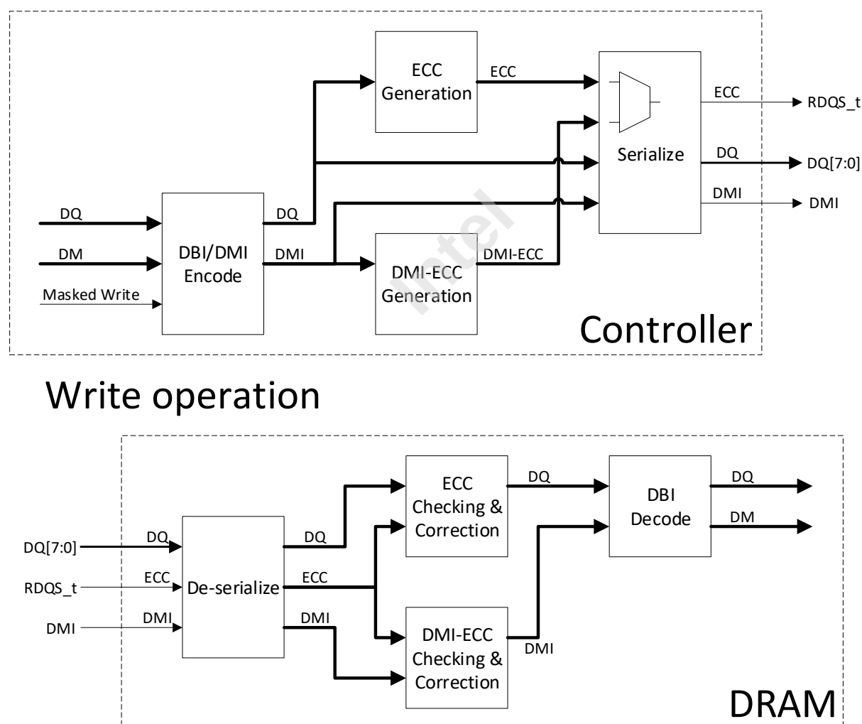
Figure 282 — Data Flow on a Memory Write Operation
