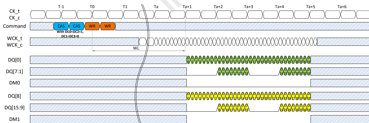
Figure 267 — Example of Write Data Copy Function Timing Diagram
