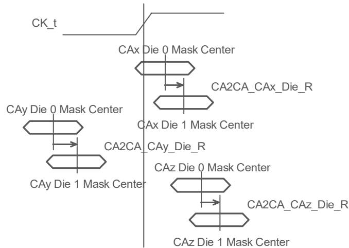
Figure 328 — CK_t Rising Edge CA Mask
