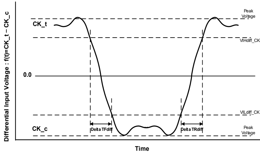
Figure 299 — Differential Input Slew Rate Definition for CK t , CK c
