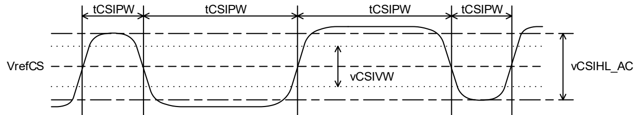
Figure 322 — Synchronous Mode CS Rx Single Pulse Definition
