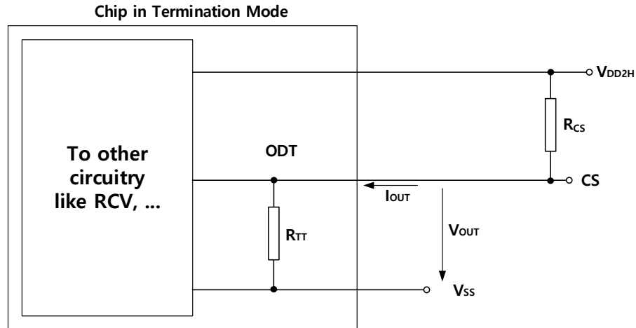
Figure 215 — On Die Termination for CS
