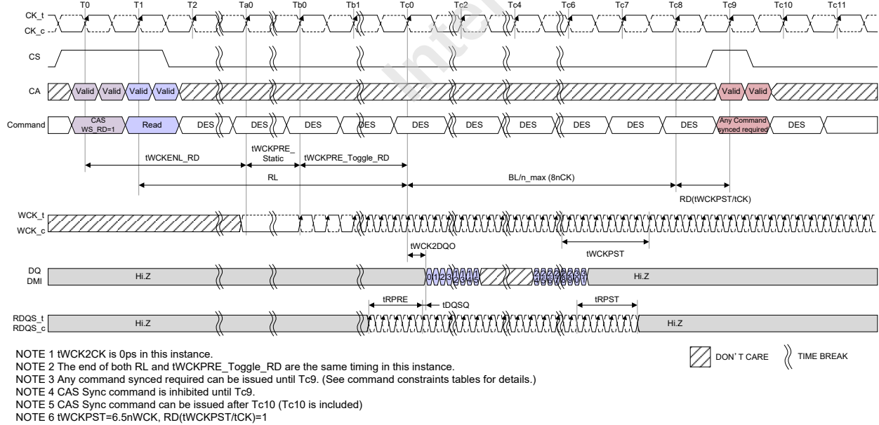
Figure 10 Read sync off timing BG Mode : CKR (WCK vs. CK) = 4:1, BL=32, tRPST=4.5nWCK
