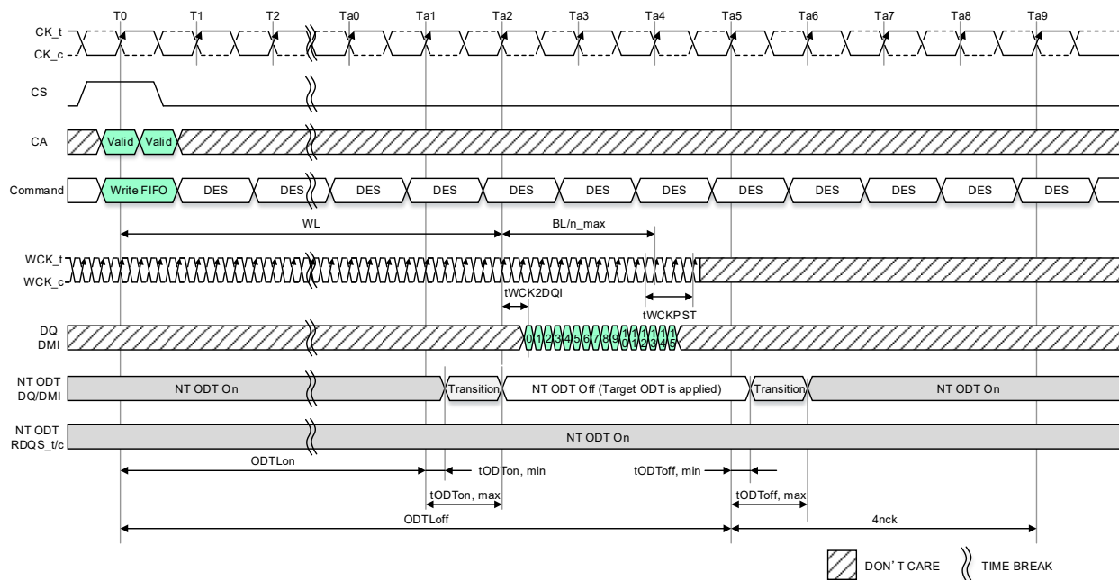
Figure 240 — Delay Time from Write FIFO to Clock Stop: 16B Mode, CKR=4:1, tWCKPST=2.5nWCK
