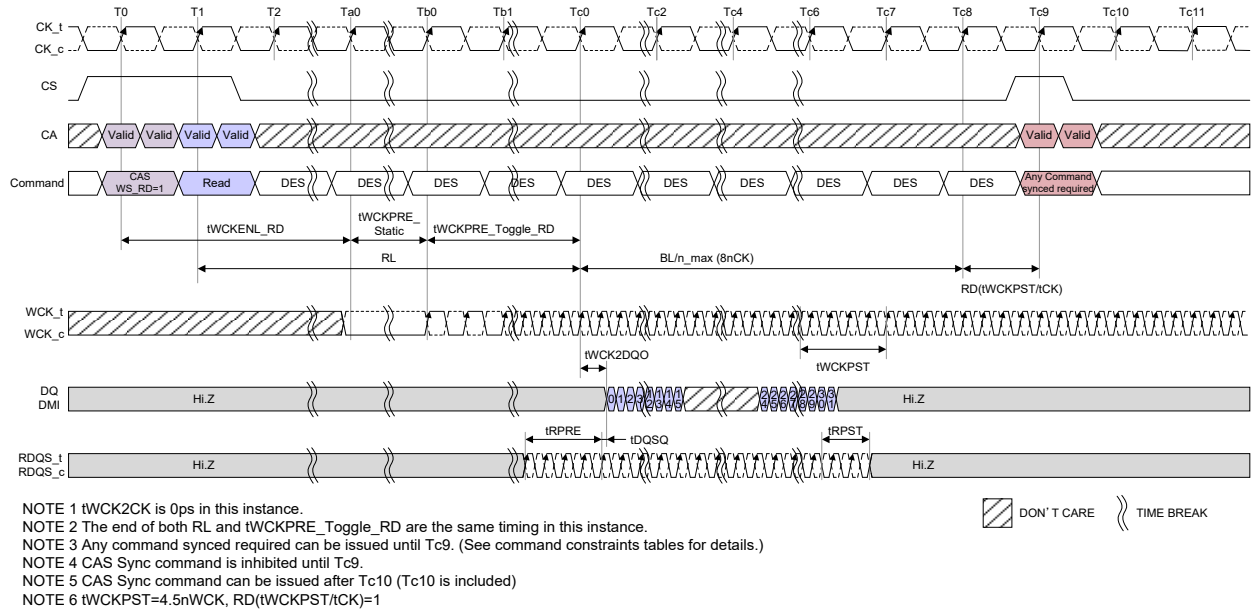
Figure 9 Read sync off timing BG Mode : CKR (WCK vs. CK) = 4:1, BL=32, tRPST=2.5nWCK
