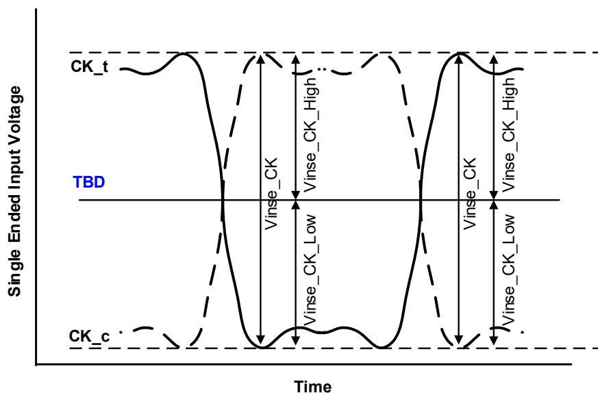
Figure 298 — Clock Single-ended Input Voltage
