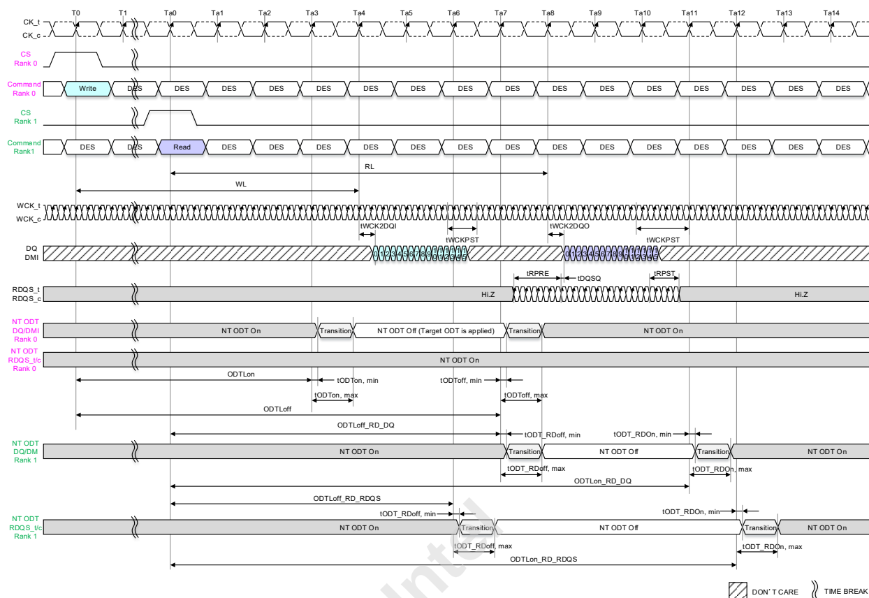
Figure 221 — Write to Read Rank2Rank Operation (MR0 OP[0]=1B)
