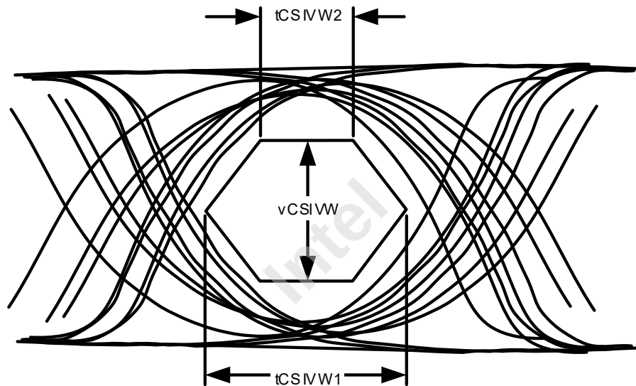
Figure 321 — Synchronous Mode CS Rx Mask Definition
