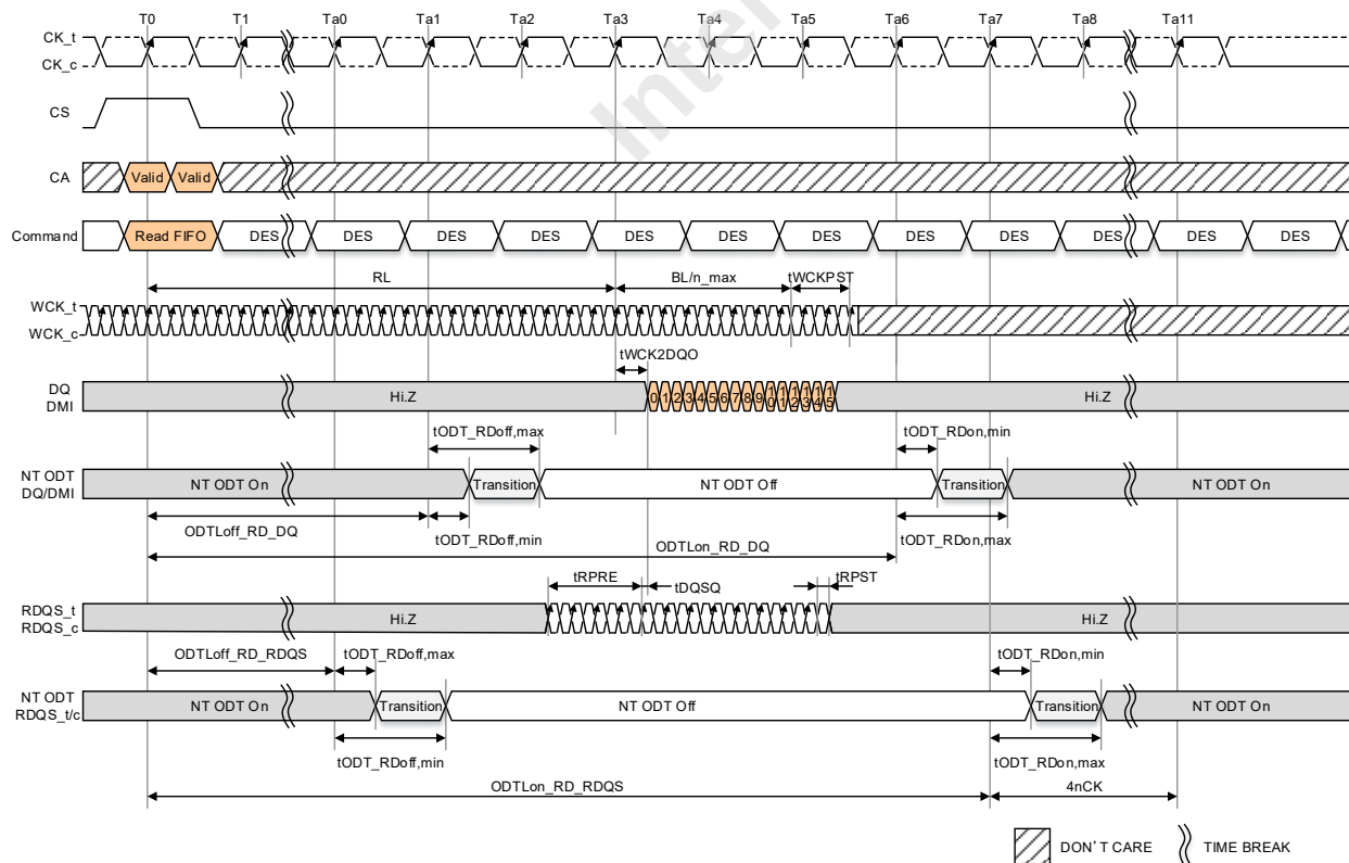
Figure 241 — Delay Time from Read FIFO to Clock Stop: 16B Mode, CKR=4:1, tWCKPST=2.5nWCK (MR0 OP[0]=1 B )
