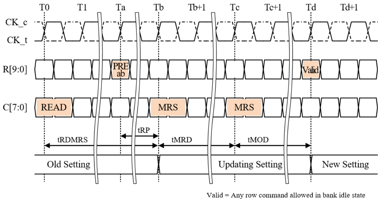
Figure 49 — Mode Register Set Timings
