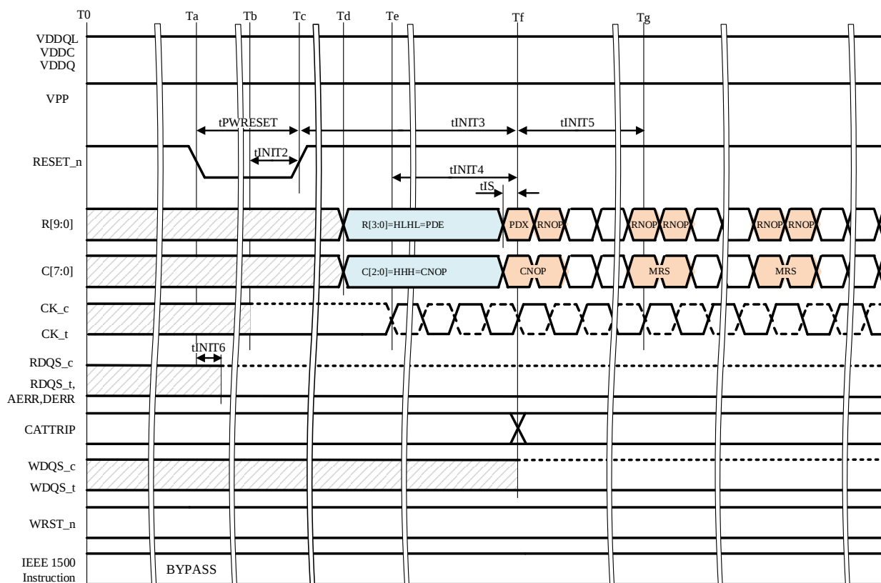
Figure 5 — HBM4 RESET and Initialization Sequence with Stable Power
