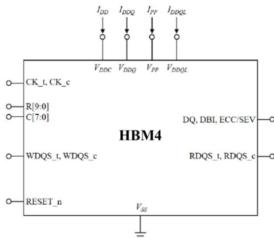
Figure 98 — Measurement Setup for IDD and IPP Measurements
