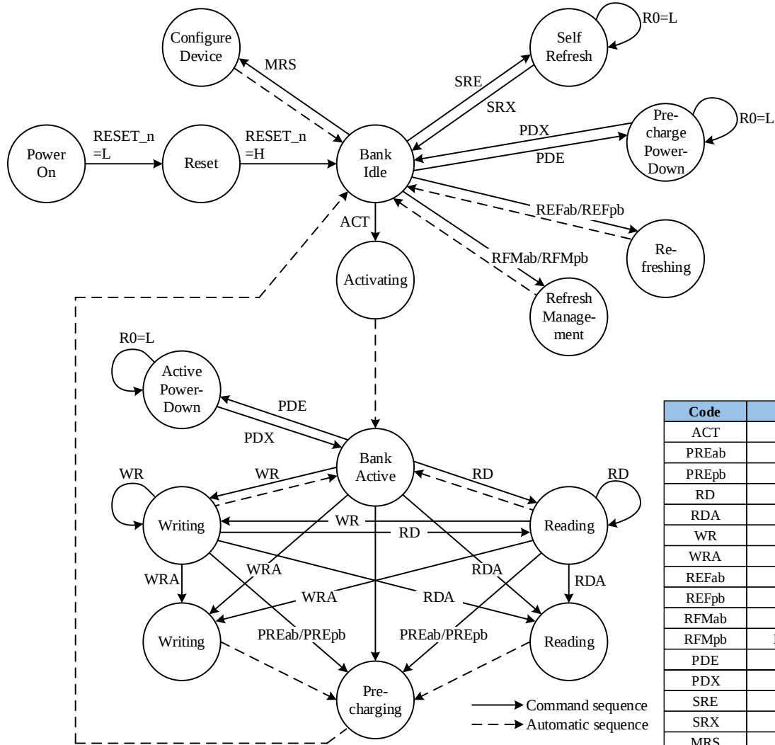
Figure 3 — Simplified State Diagram
