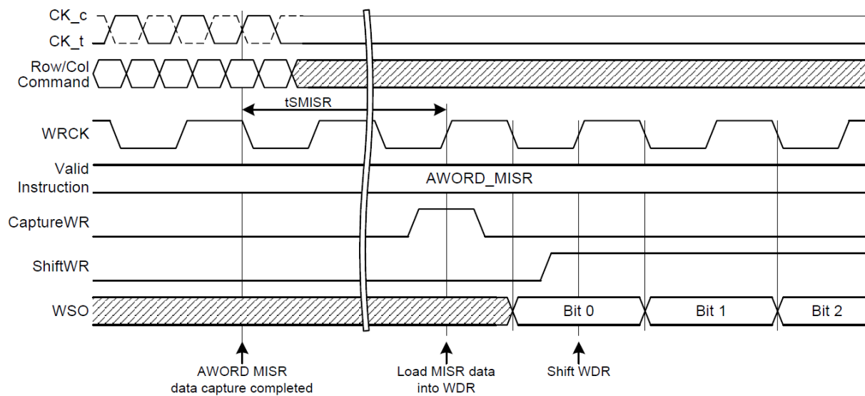
Figure 115 — IEEE1500 DWORD_MISR / AWORD_MISR Instruction Related Timings
